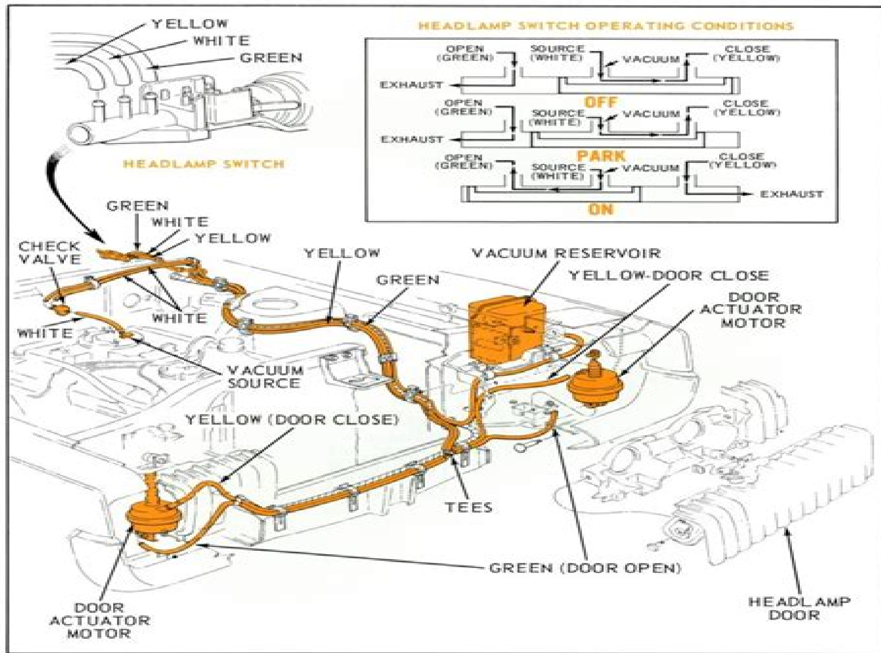
Fig. 34 - 1968 Cougar Vacuum Operated Headlamp Doors
