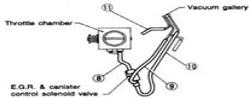
VIEW A
