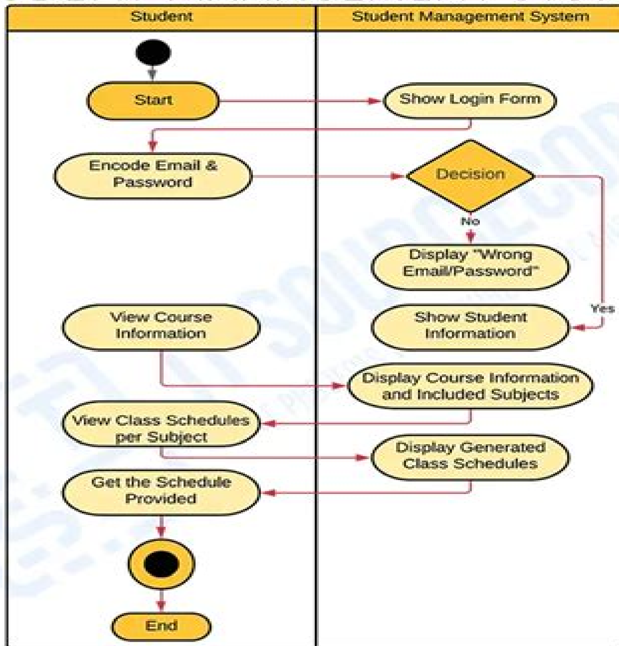
ACTIVITY DIAGRAM
