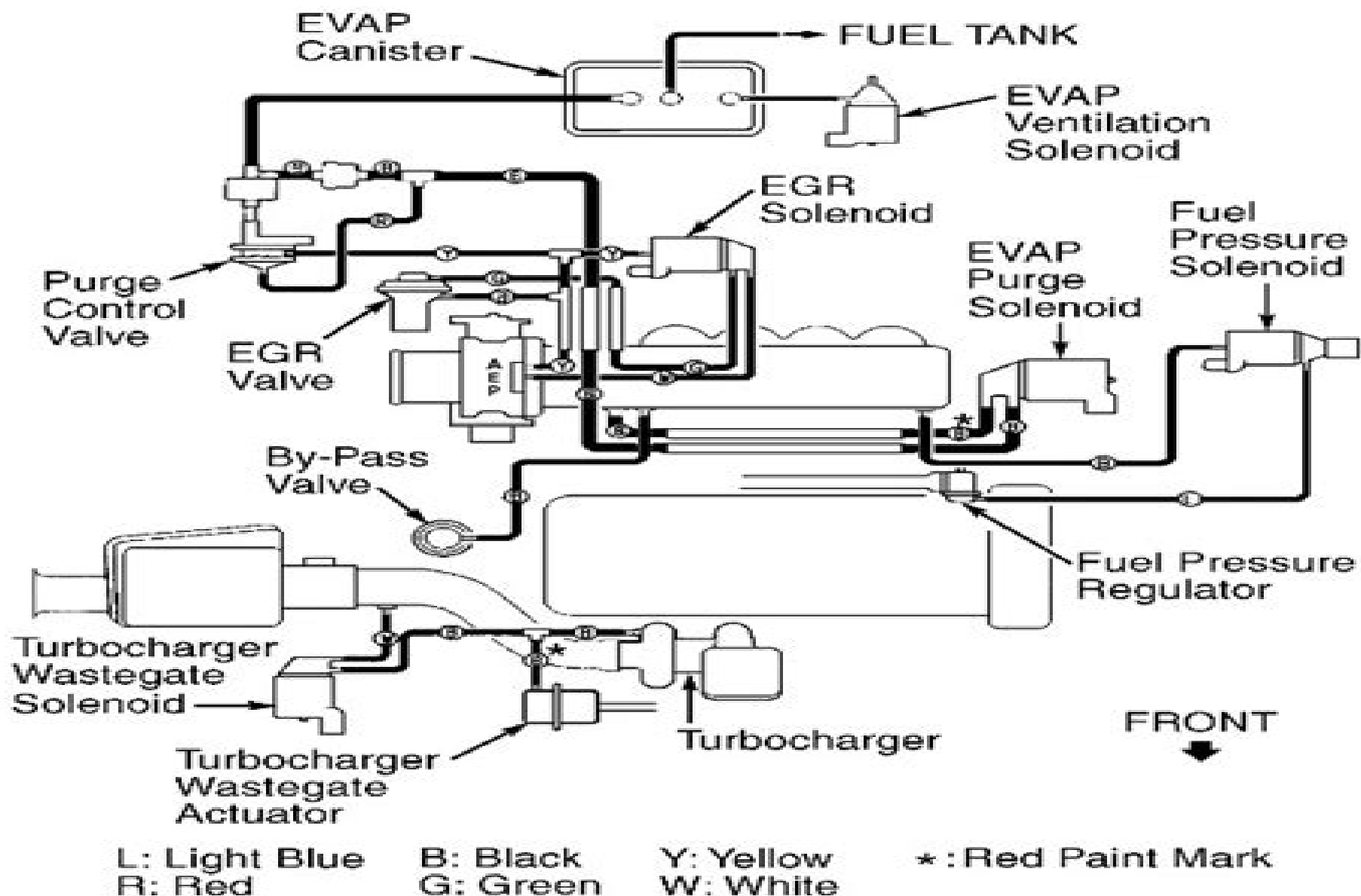
Fig 3: Vacuum Diagram (Eclipse 2.0L Turbo)
