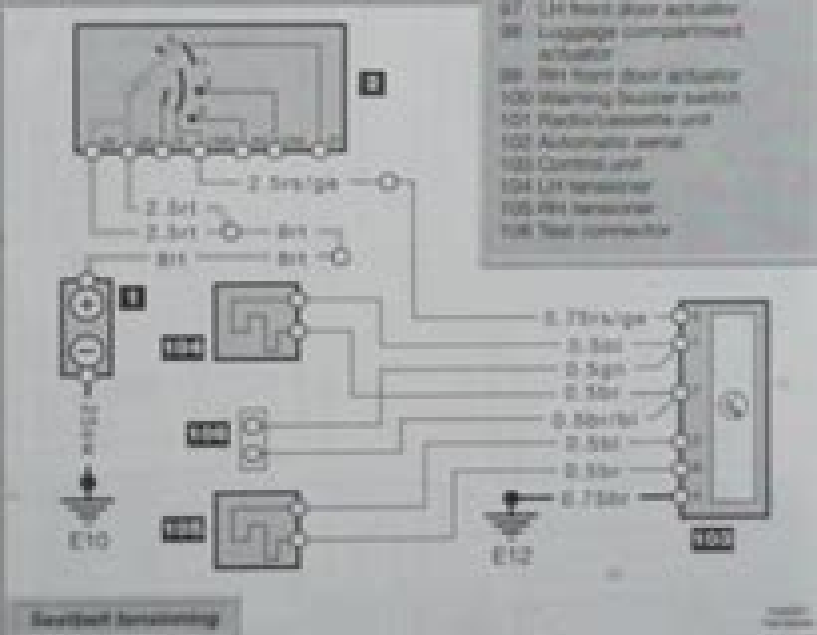
Diagram 8 : Electric mirrors, central locking radio/cassette and seatbelt tensioner
