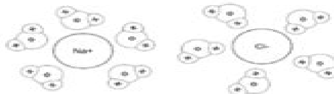
Figure 3: Hydration Spheres
