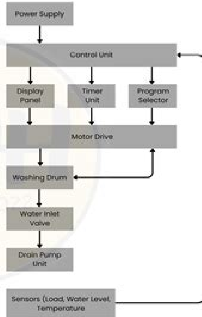
Block Diagram of Washing Machine with Explanation
