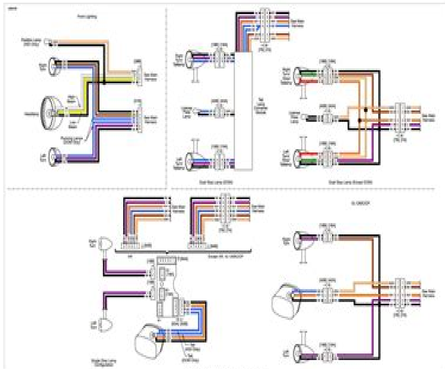
Figure 8-11: Lighting (1965-1966 Mustang)
