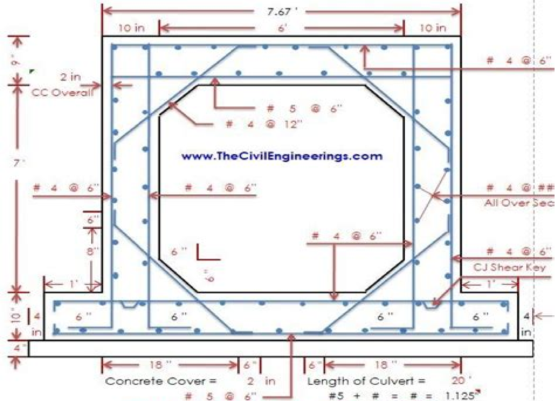
TYPICAL SECTION OF BOX CULVERT ( 6 X 7 )
