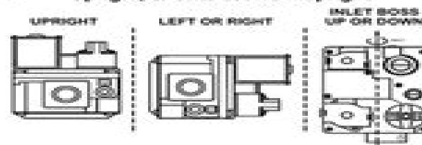
Figure 1. Gas valve mounting positions
