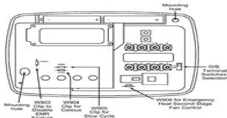
Figure 1. Thermostat base
