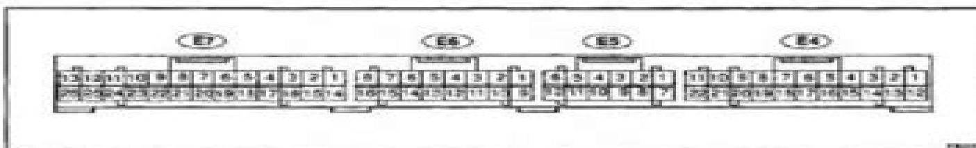
Terminals Of ECM - Connector View
