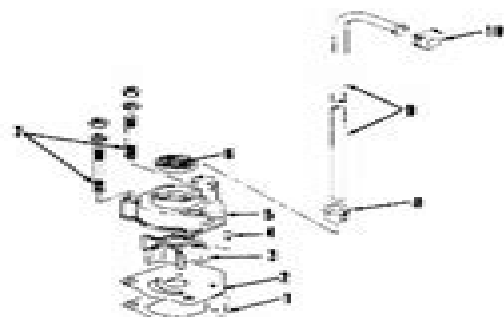
Fig. S27-14—Exploded view of water pump assembly.
