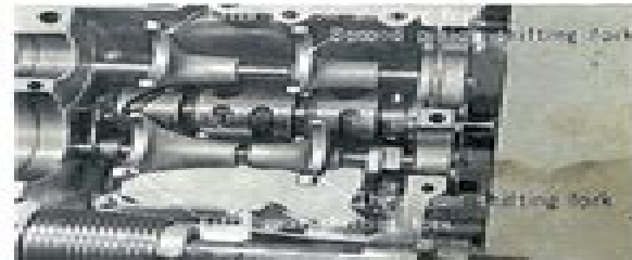
Fig. 6-8-5. Fitting shifting forks
