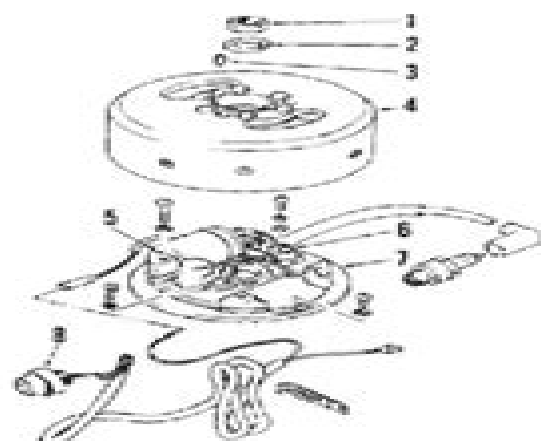
Fig. S21-3—Exploded view of magneto.
