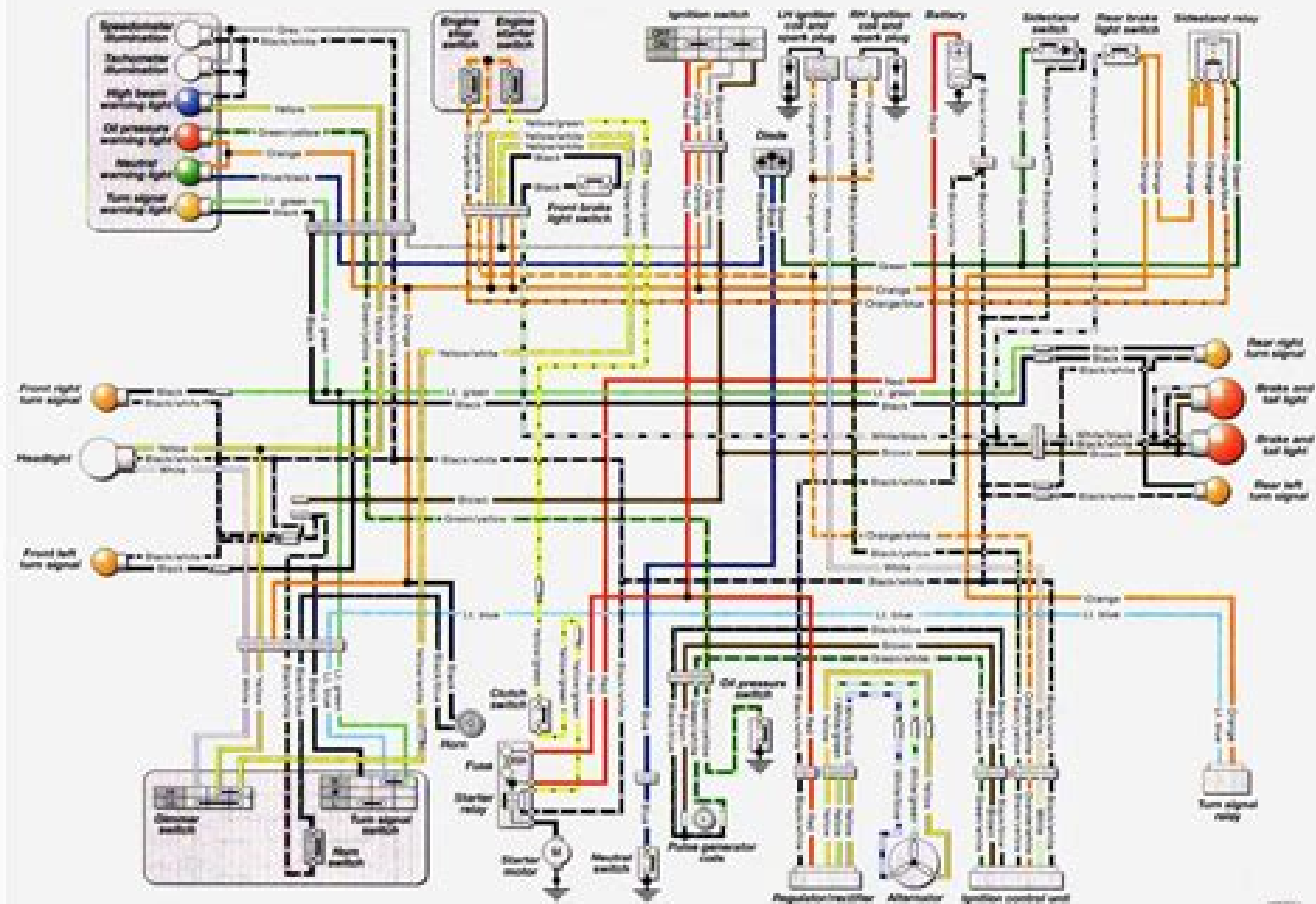
Wiring diagram - US G5500 EV model
