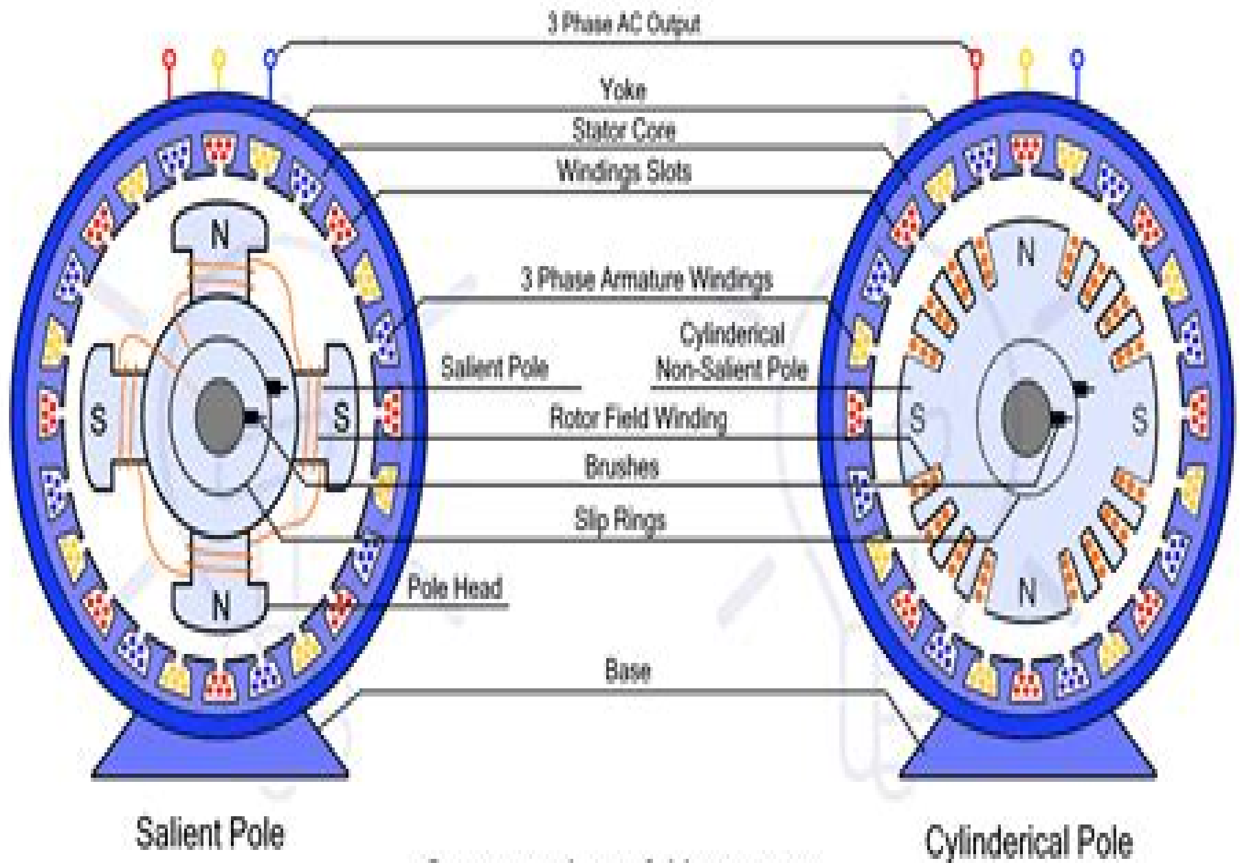
Construction of Alternator
