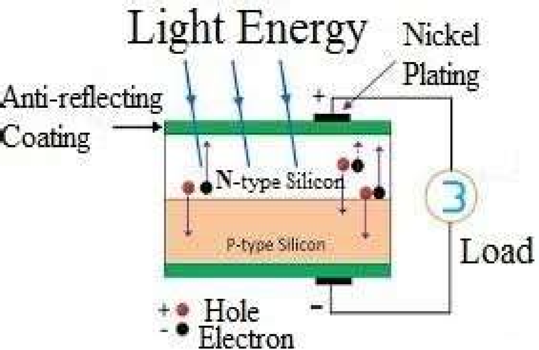
Construction of Solar Cell
