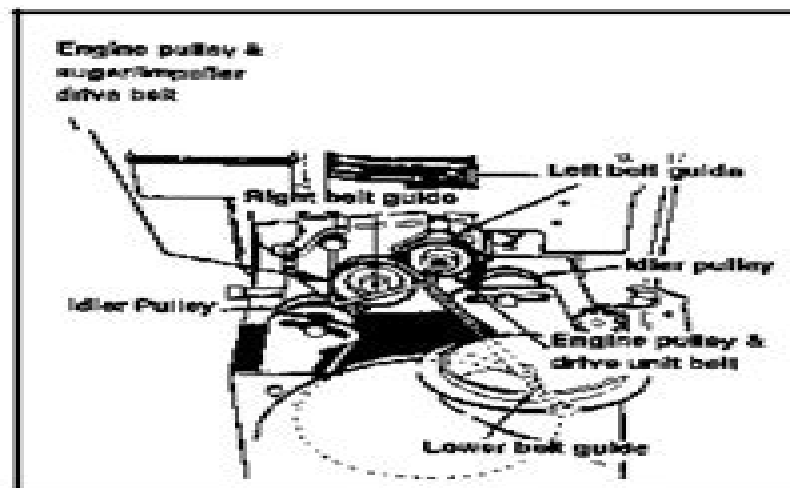
Figure 11. Drive Belts and Pulleys - Belt Cover Off
