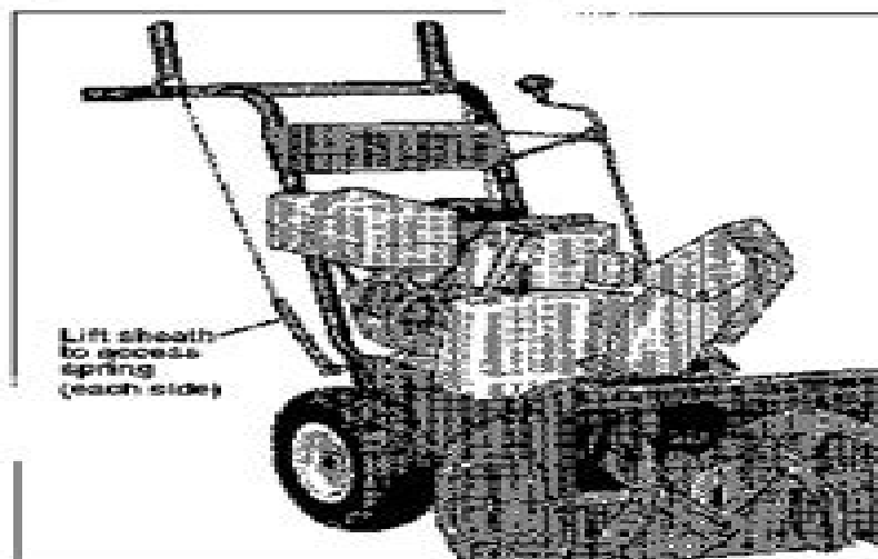
Figure 12. Drive Control Spring
