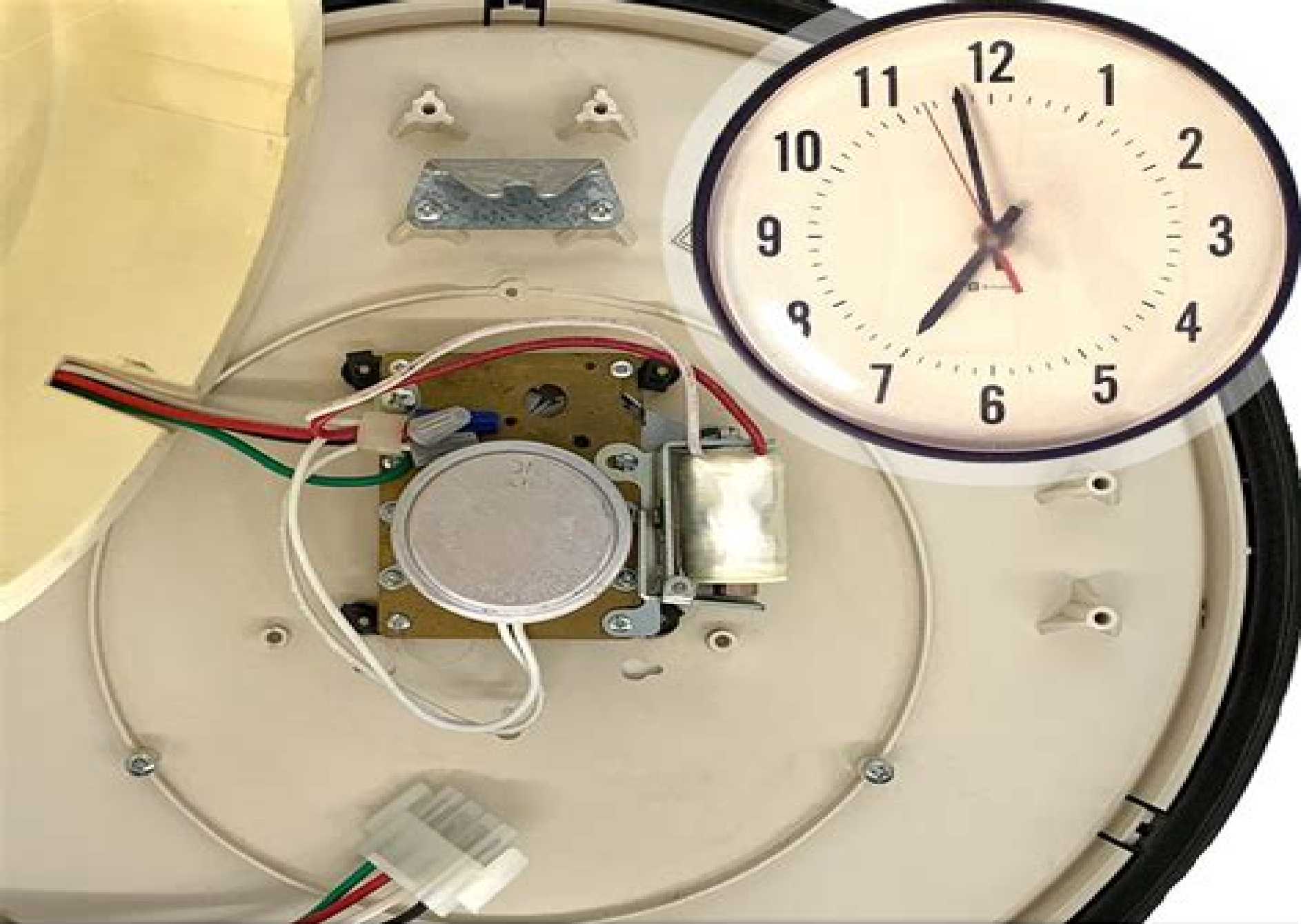
3-Wire Movement (9200 SERIES)
