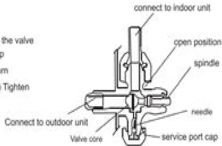
3-way valve diagram
