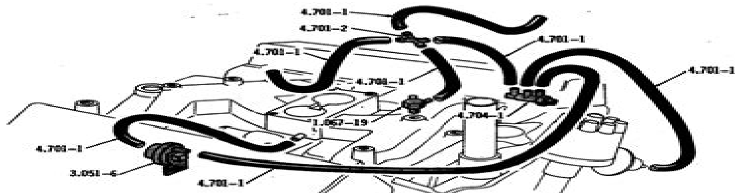
VACUUM ADVANCE MODULATION SYSTEM . . . 10-25-45 (360-WHDC-E/CALIF), 1974 80 (V8-E/CALIF), 1975 80 (V8-CALIF)
