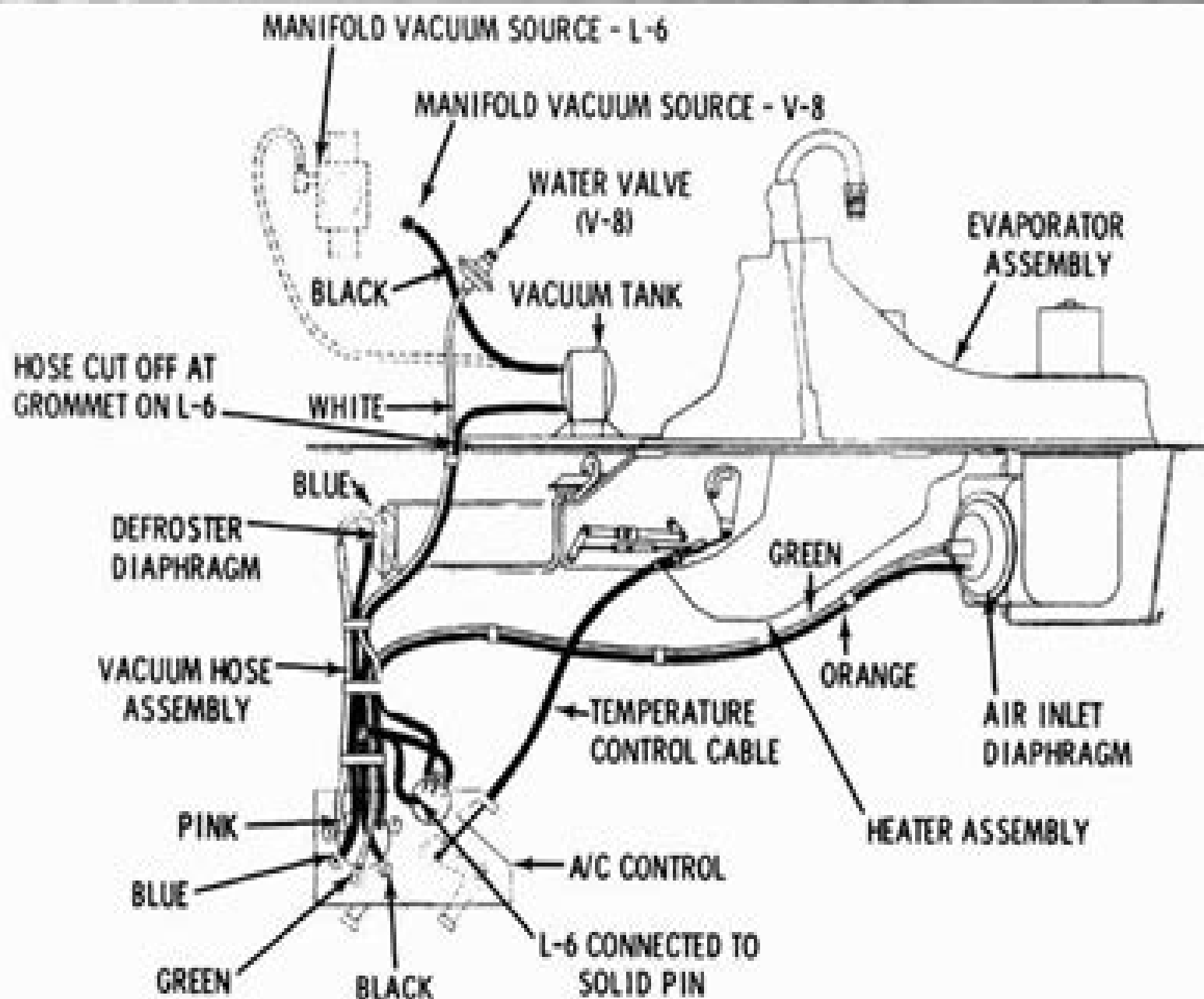
Fig. 1C-23—Vacuum Hose Routing
