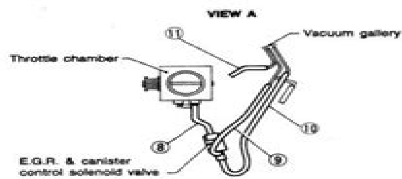
1.7n Vacuum hose routing diagram for 1991 through 1994 MPFI models with the SR20DE engine
