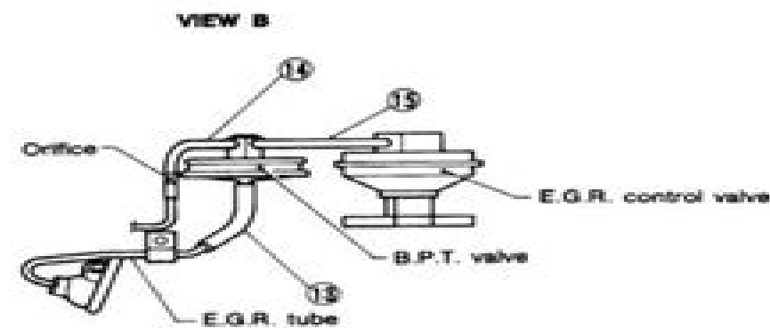
1.7n Vacuum hose routing diagram for 1991 through 1994 MPFI models with the SR20DE engine
