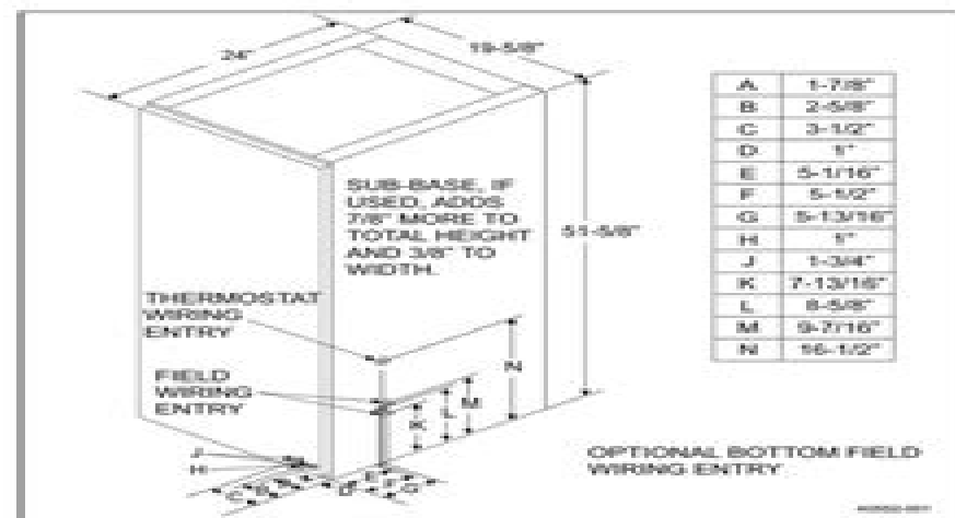
FIGURE 1: Furnace Dimensions
