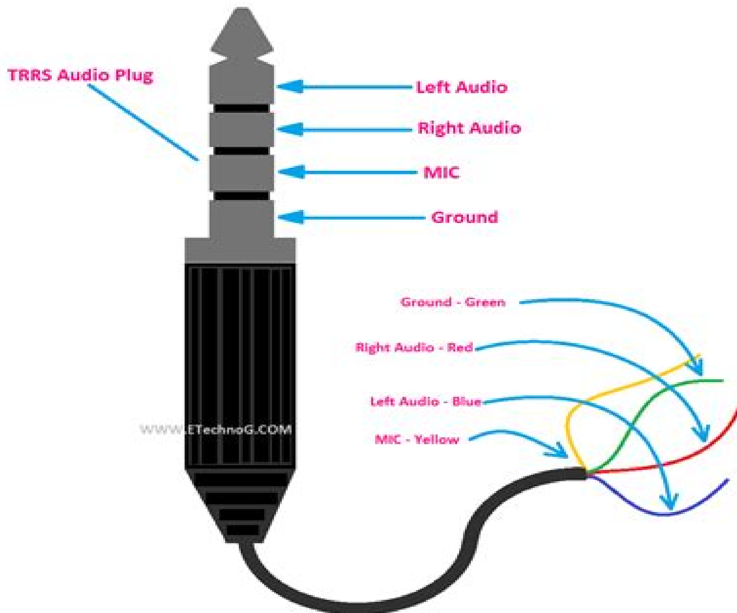
Headphone Jack Pinout and Color Codes
