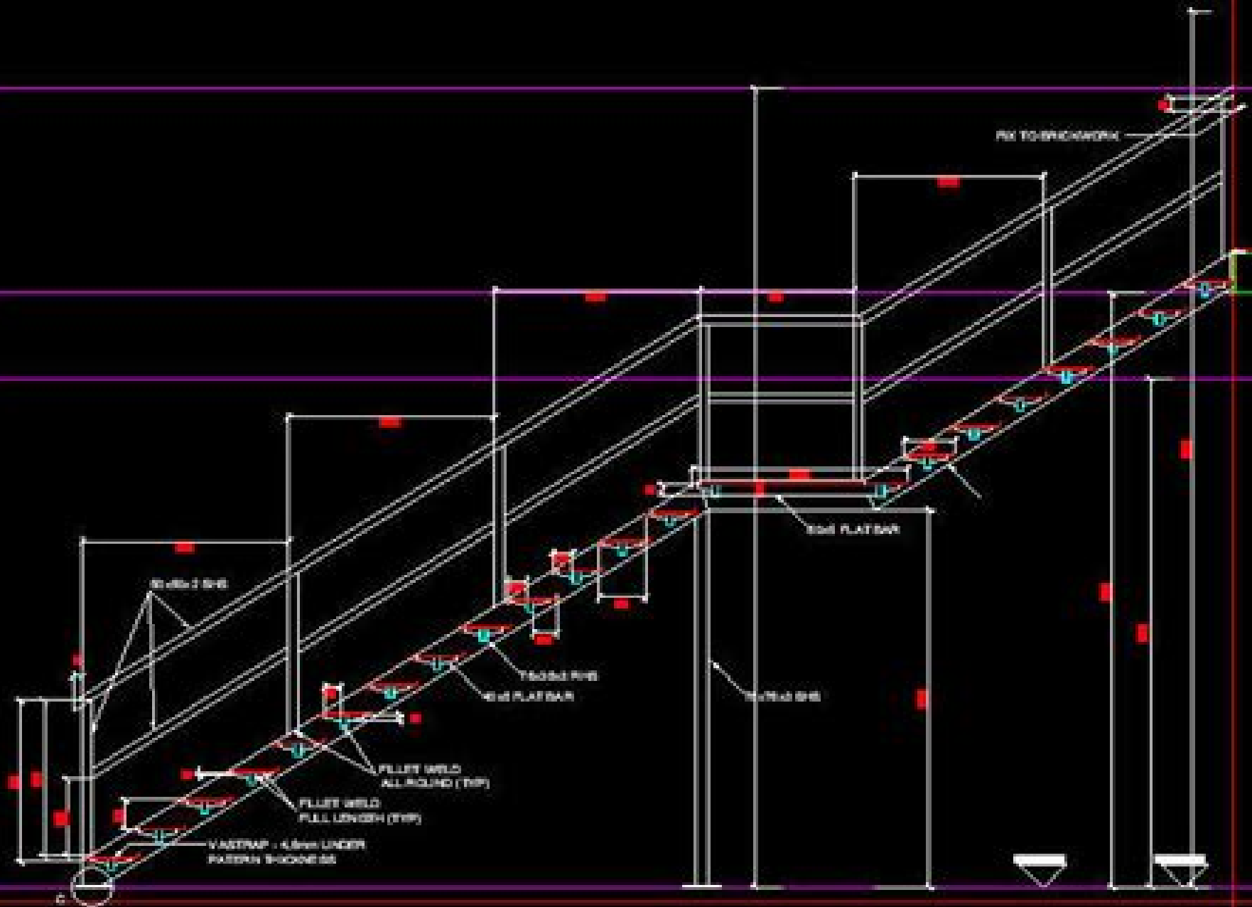
— DETAIL SECTION - STEEL STAIRCASE Scale 1:10
