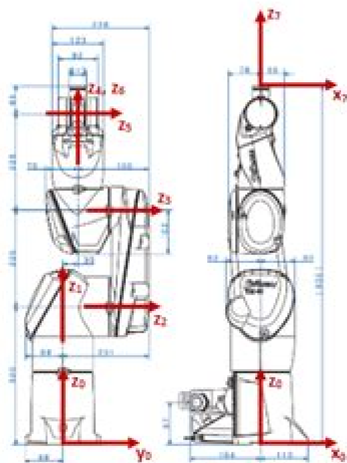
Figure 3: (a) The Staubli TX-40 robotic arm; (b) Joint axes and dimensions. All dimensions are in millimeters. Joints are numbered consecutively from 1 to 6. Frame {0} is the space frame. Frame {7} is the end-effector frame. Note: the schematic does not show joint frames – only the joint axes ( z_1, z_2, \dots, z_6 ). Recall that joint frames are not needed to calculate the kinematics with the Product of Exponentials Formula.
