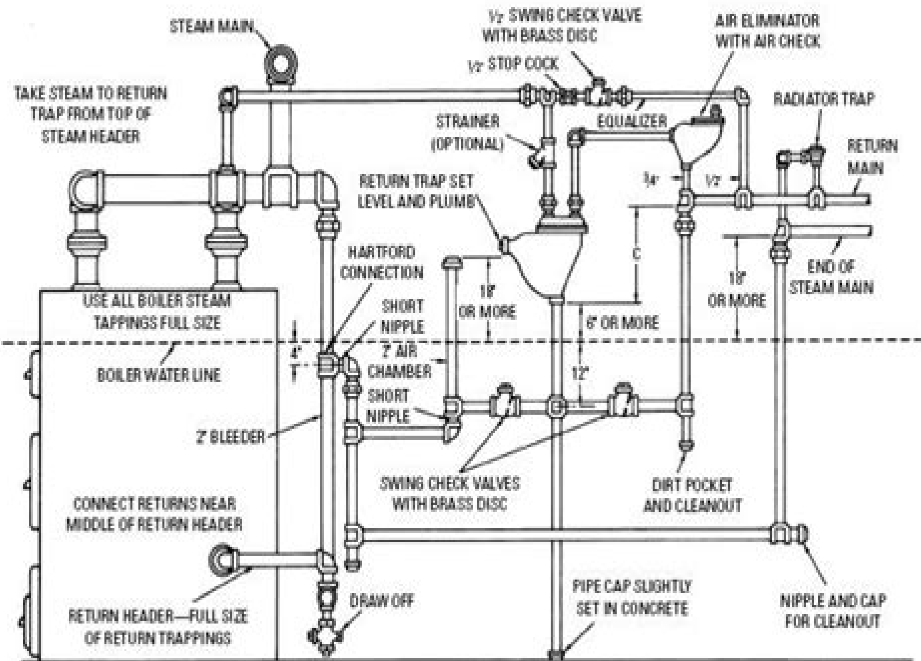
Figure 10-38 Boiler piping of a return-trap steam heating system. (Courtesy Durham-Bush, Inc.)
