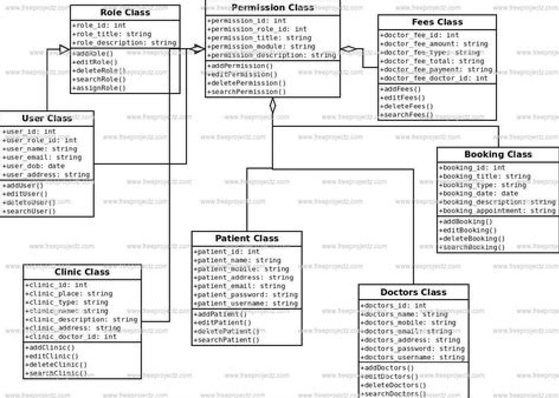
Class Diagram of Doctor Appointment System
