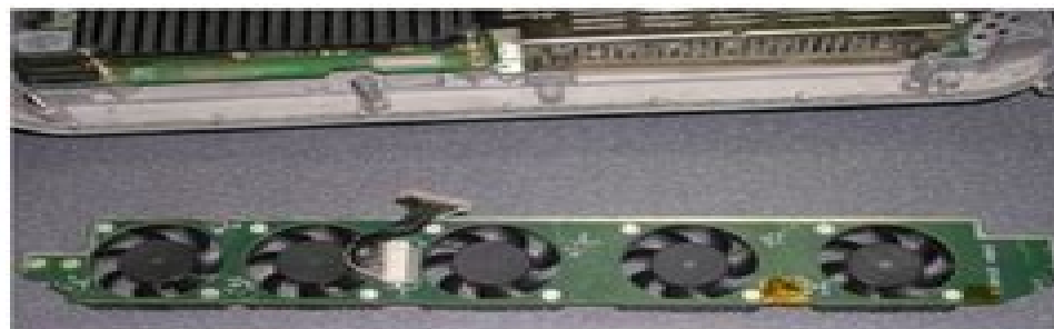
Figure 8-68 Disconnecting the Fan Cable from the BEP
