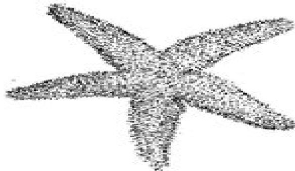
Figure 1 -Aboral Surface
