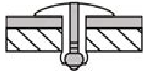
Large Flange
