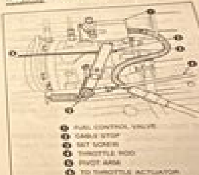
Throttle Actuator Lever Bracket — First Arm Configuration
