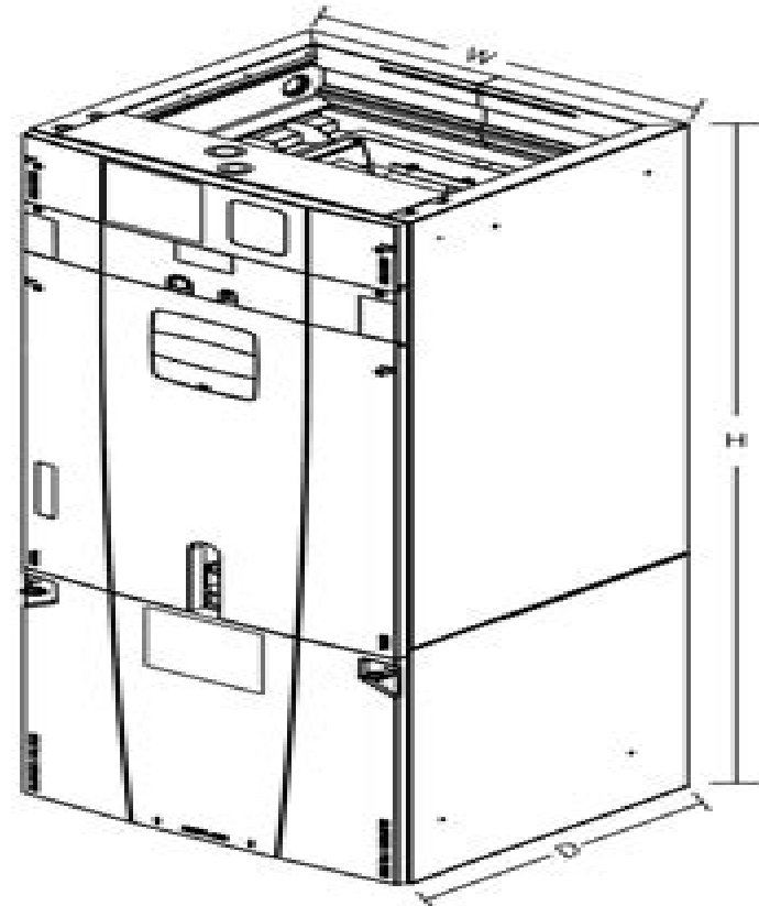
TAM7 AIR HANDLER DIMENSIONAL DATA
