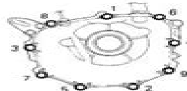
[Crankcase Cover Tightening Sequence]
