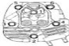
[Cylinder Head Tightening Sequence]
