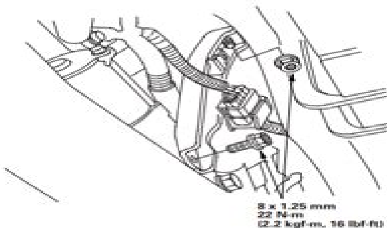
K20Z3 engine
