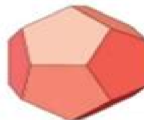
Dodecahedron
