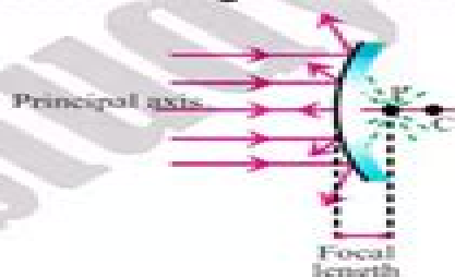
Reflection of light on convex mirror
