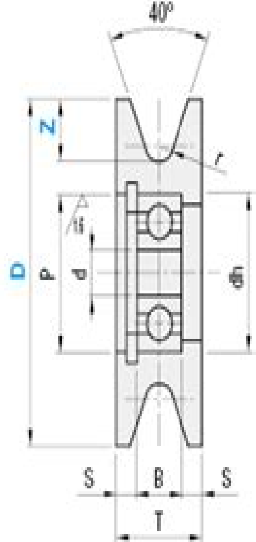
Sheave (for Wire Cable)
