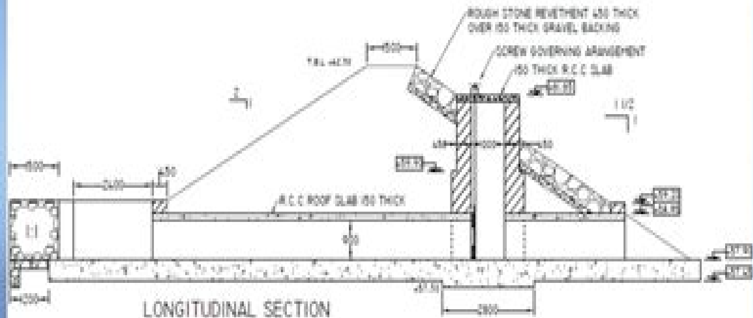
TANK SLUICE WITH TOWER HEAD
