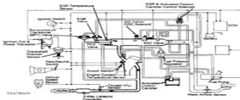
Fig. 1: Vacuum Diagram (Altima) Courtesy of Nissan Motor Co., U.S.A.
