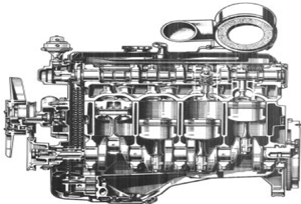
Fig. A-1 Sectional view of the engine.
