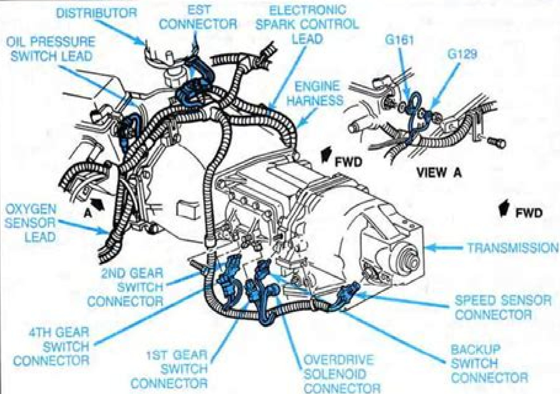
Fig. 8A-26 — Manual Transmission Wiring
