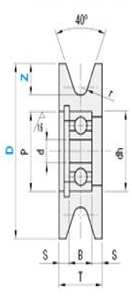
Sheave (for Wire Cable)
