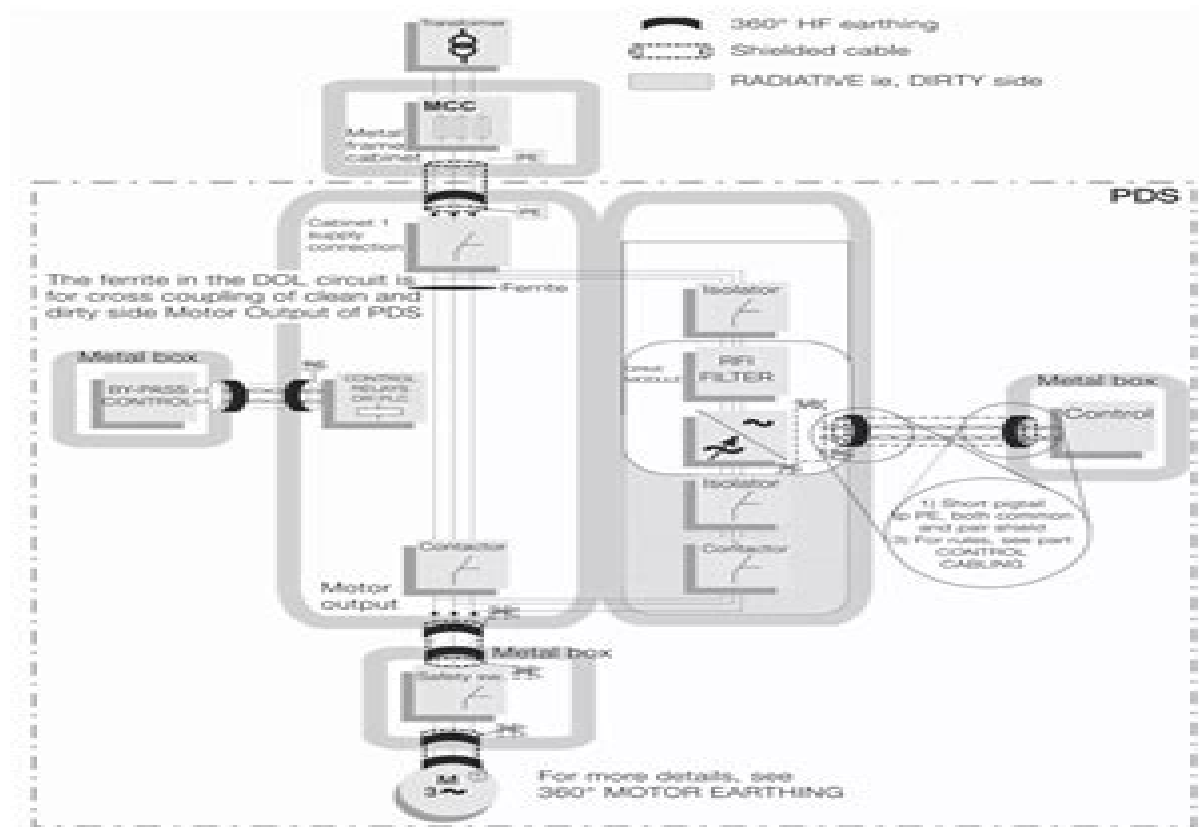
Figure 4-3 Basic scheme with by-pass.
