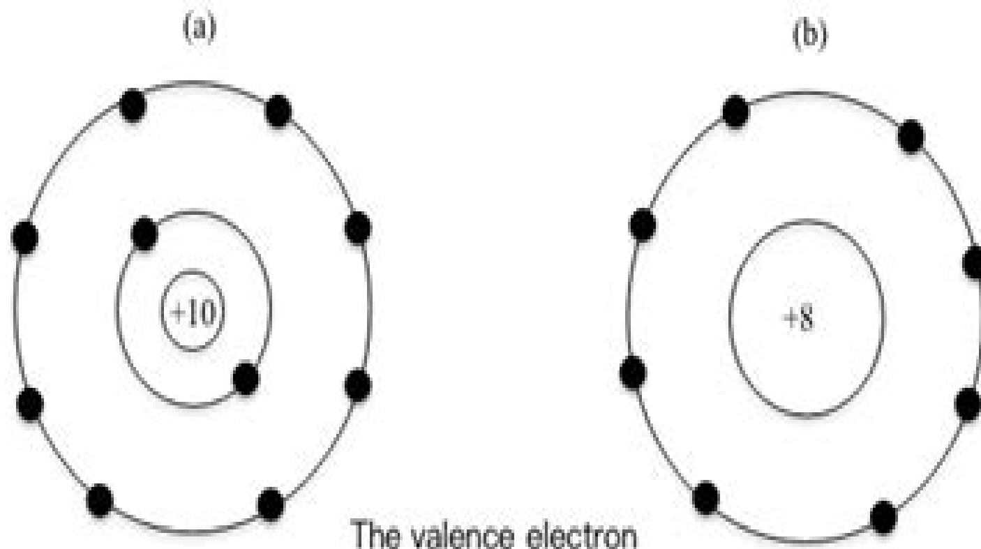
Figure 3. Diagram of a Ne atom using the shell model (a) and the core charge concept (b).
