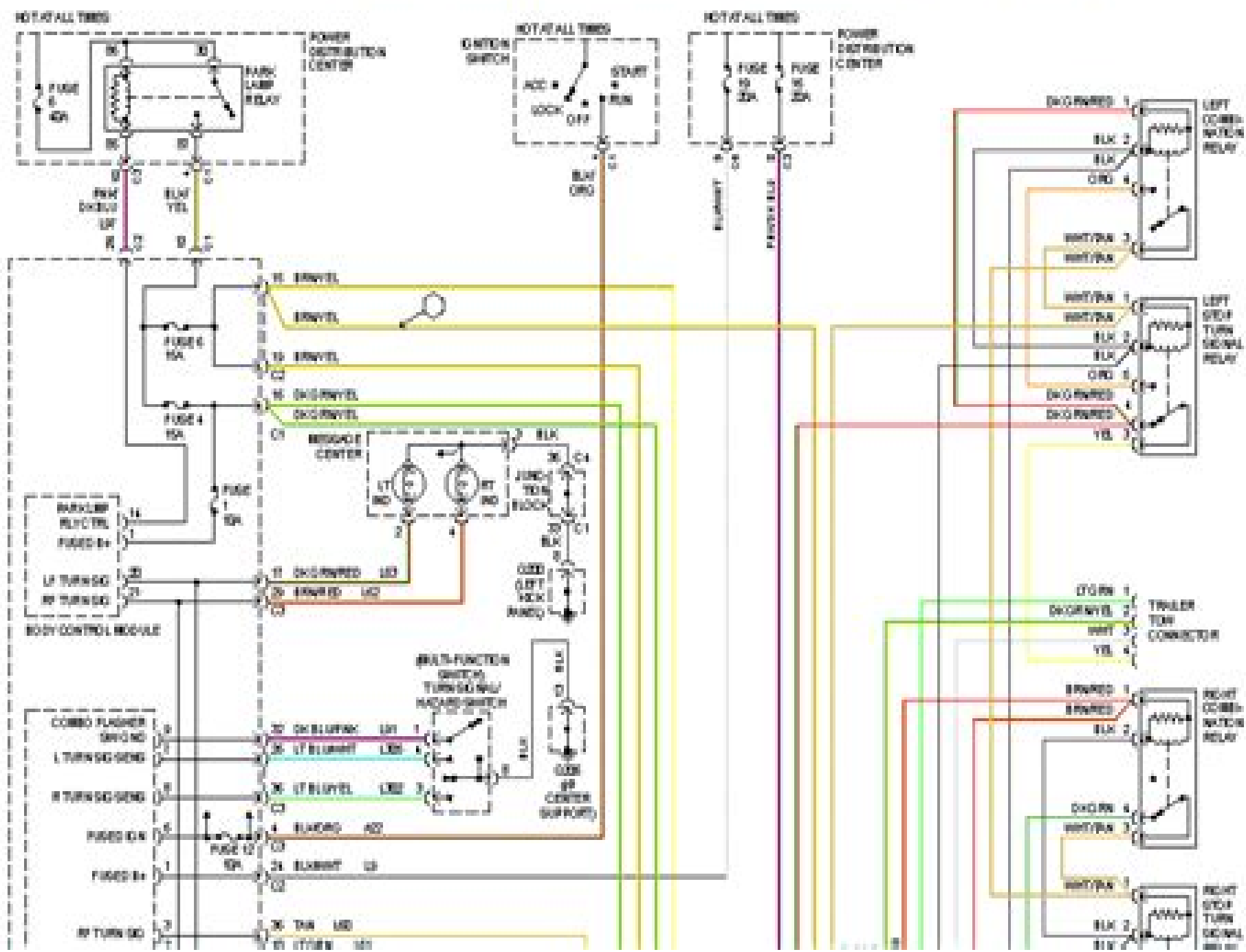
1997 Dodge Grand Caravan SE-Fig. 24: Exterior Lamps Circuit, W/ Trailer Tow
