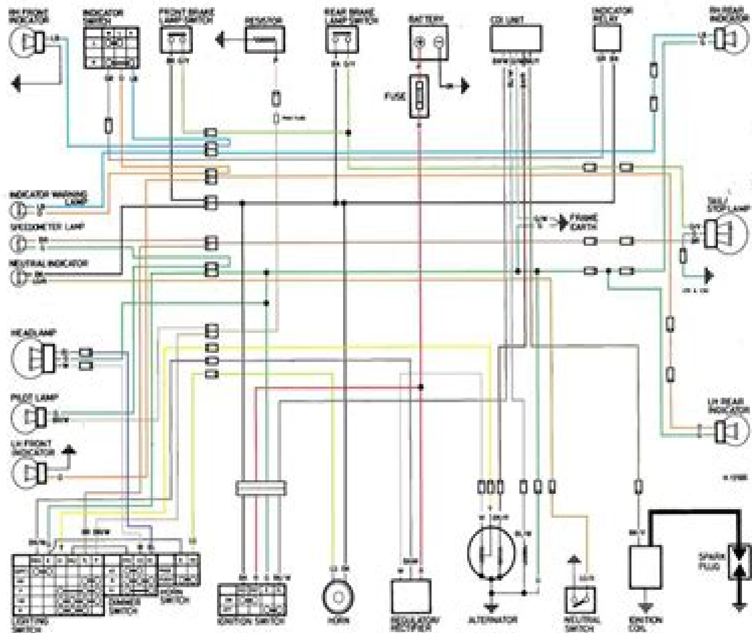
Wiring diagram - C50-C, C70-C and C90-C models
