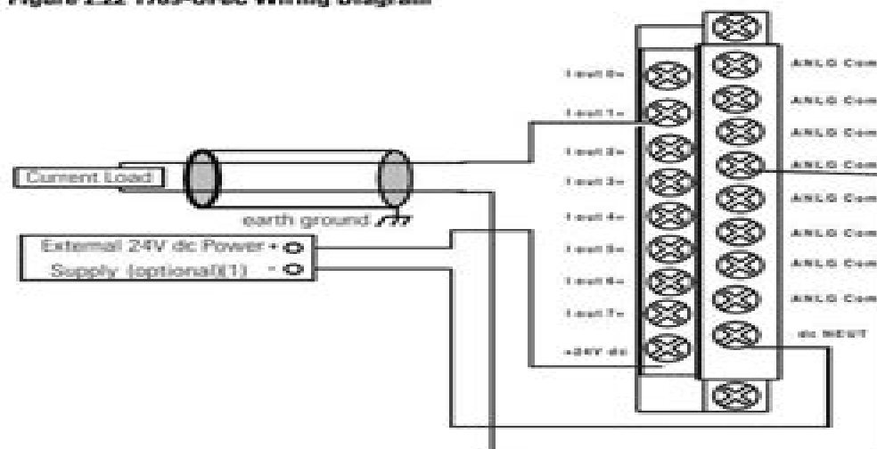
Figure 2.22 1769-OFBC Wiring Diagram
